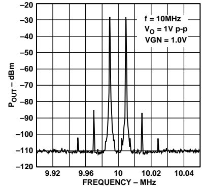
Figure 21. Intermodulation Distortion
