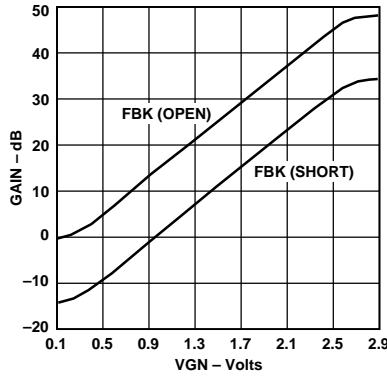
Figure 2. Gain vs. VGN for Different Gain Ranges
