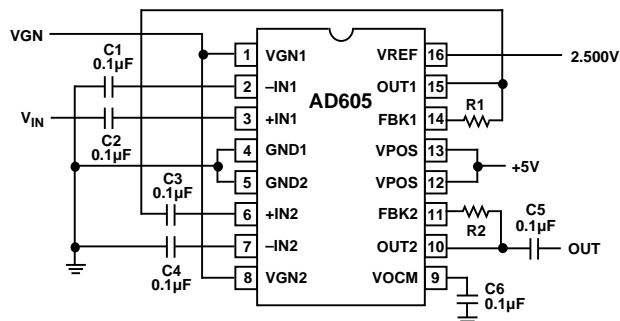
Figure 37. Doubling the Gain Range with Two Amplifiers
