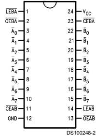
Pin Assignment for DIP and Flatpak
