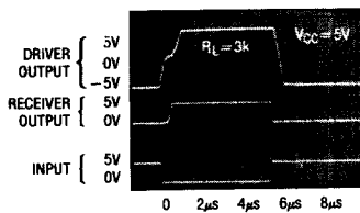
Output Waveforms
