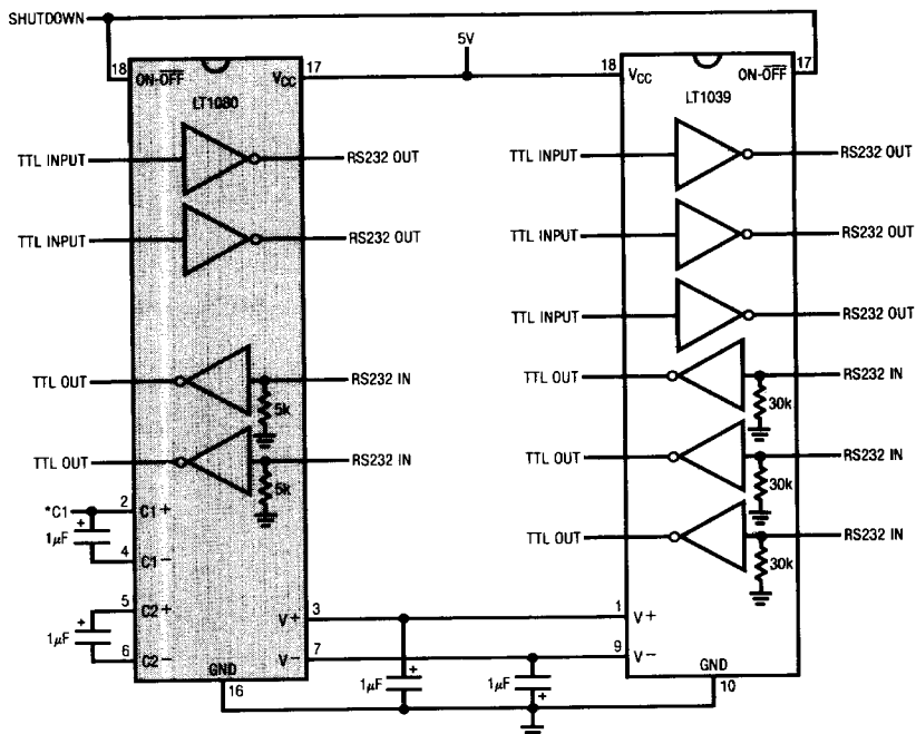
Supporting an LT1039 (Triple Driver/Receiver)
