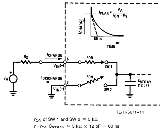
FIGURE 3. Analog Input Impedance
