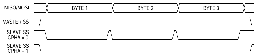
Figure 13-5. \overline{SS} Timing
