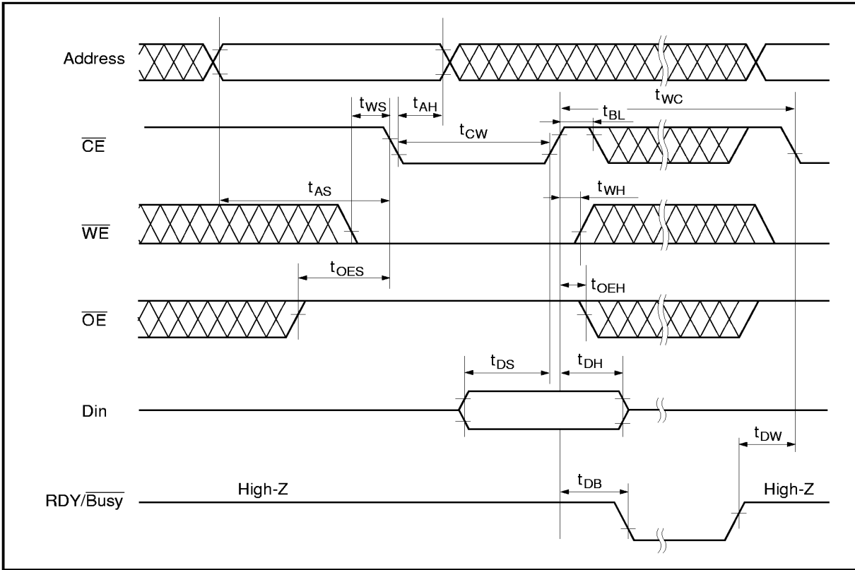
Byte Write Timing Waveform (2) ( \overline{\text{CE}} Controlled)
