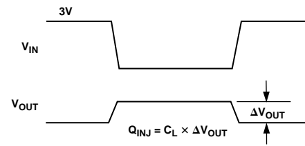
6. Charge Injection
