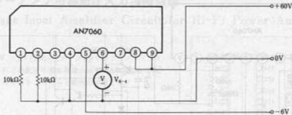
Test Circuit 4 ( V_{6-4(D)} )
