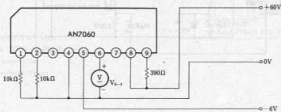
Test Circuit 5 ( V_{6-4(D)} )
