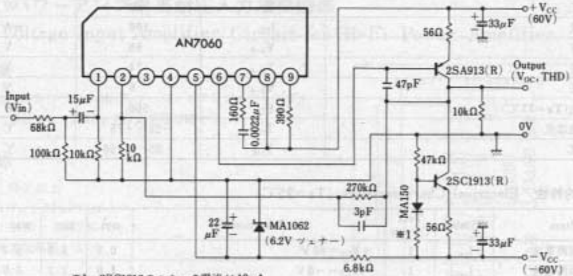
Test Circuit 2 ( V_{oc} , THD(1), THD(2))
