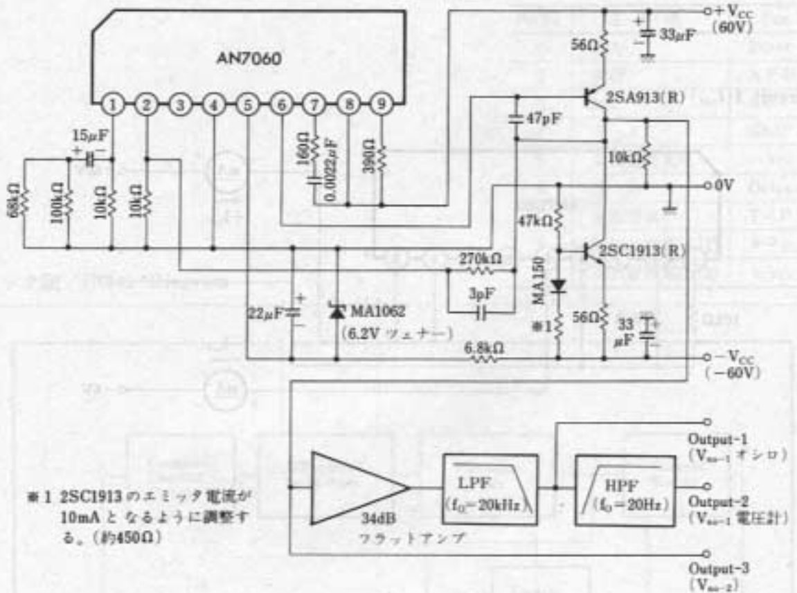
Test Circuit 3 ( V_{in} )
