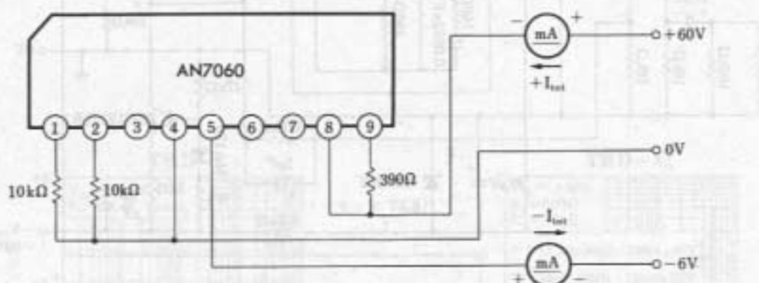
Test Circuit 1 ( I_{tot} )
